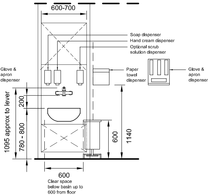
Elevation lever tap
