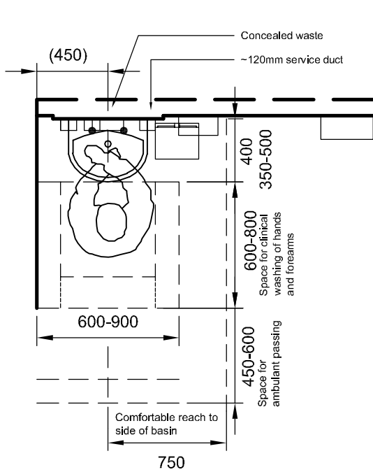
Concealed services flush with the wall finish
